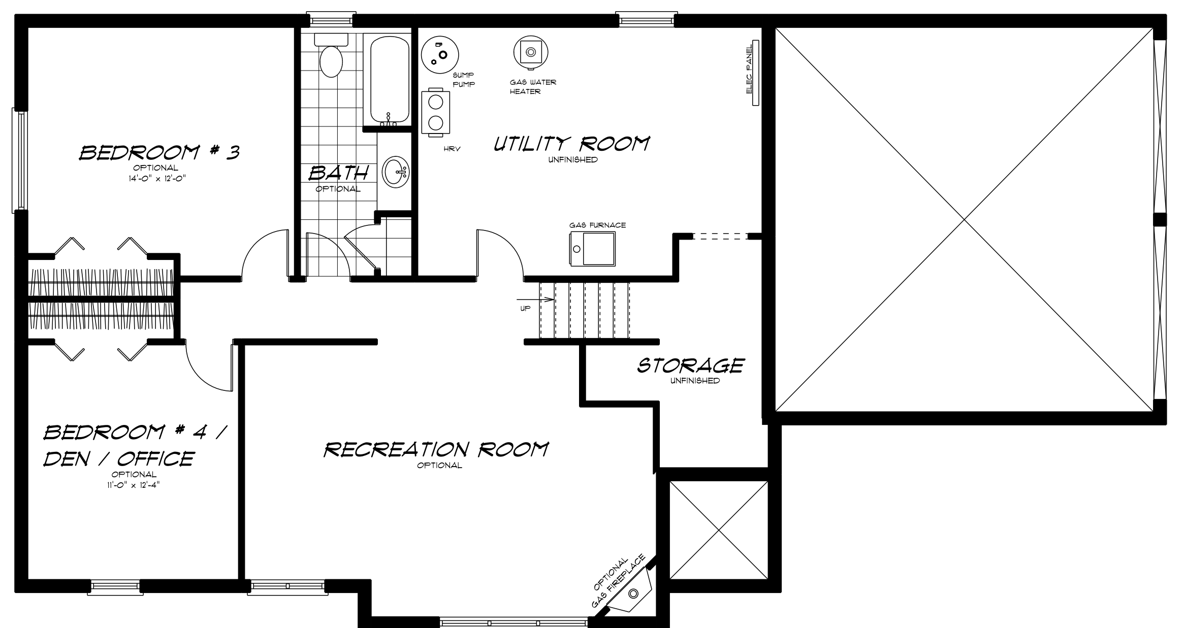
LOWER FLOOR PLAN
