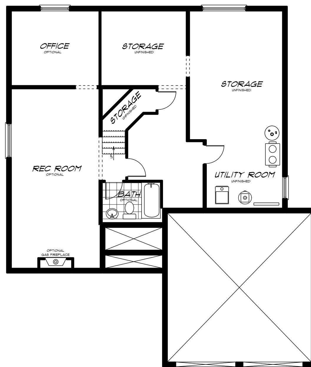
BASEMENT PLAN
