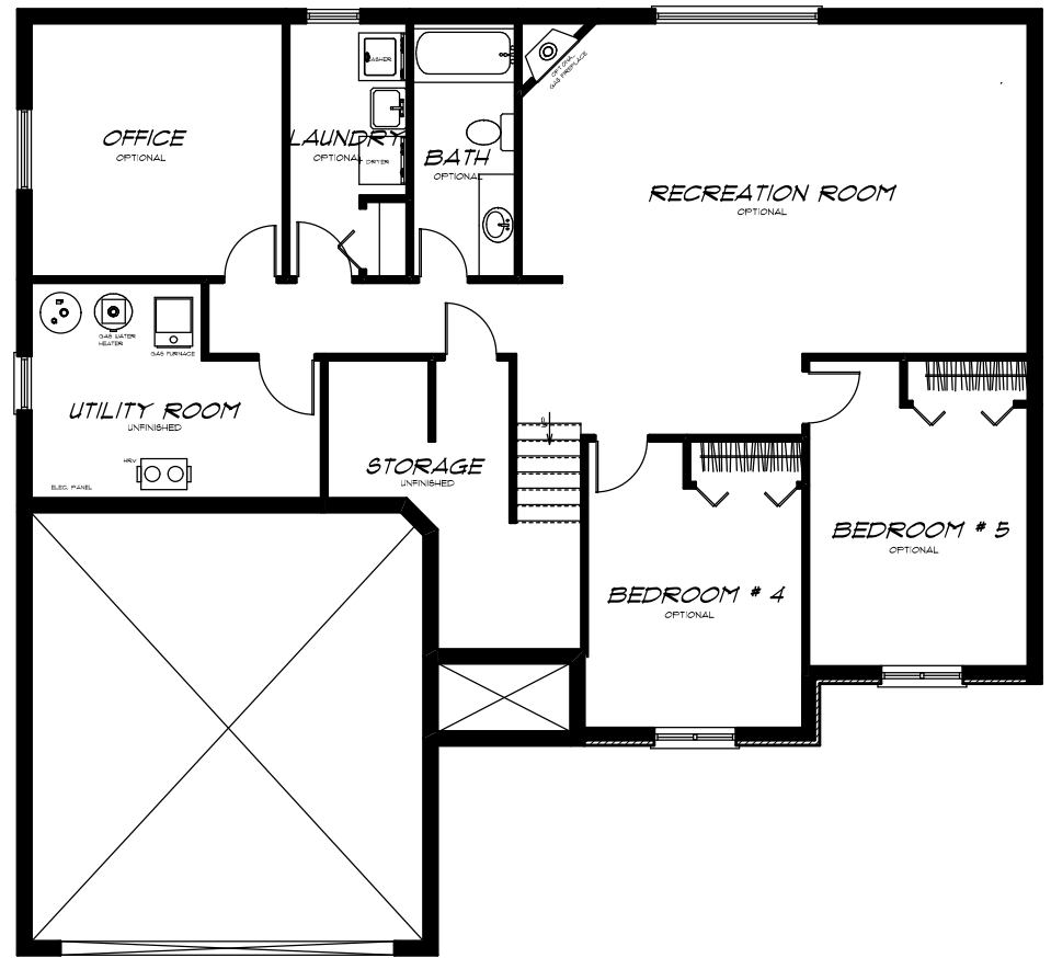
LOWER FLOOR PLAN
