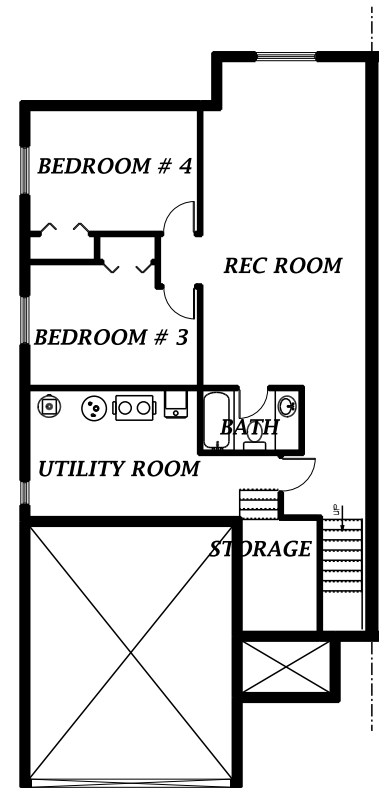
OPTIONAL FINISHED LOWER LEVEL VERSION 'B' 770 SQ.FT.
